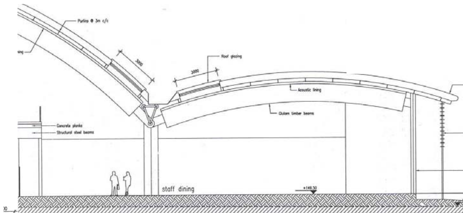
Original Valley Gutter
